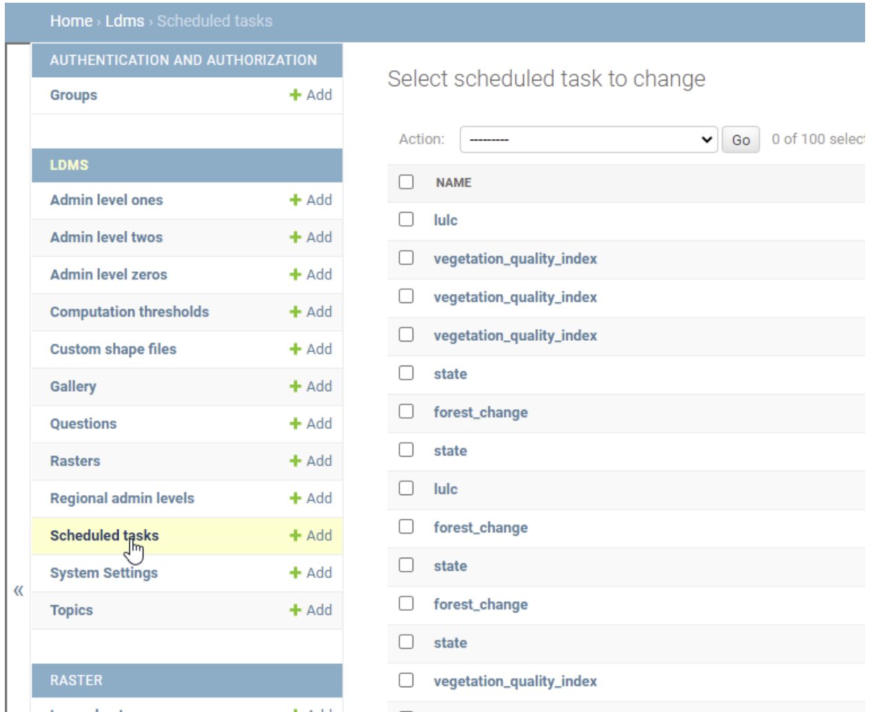
Fig. 7: Schedule task
