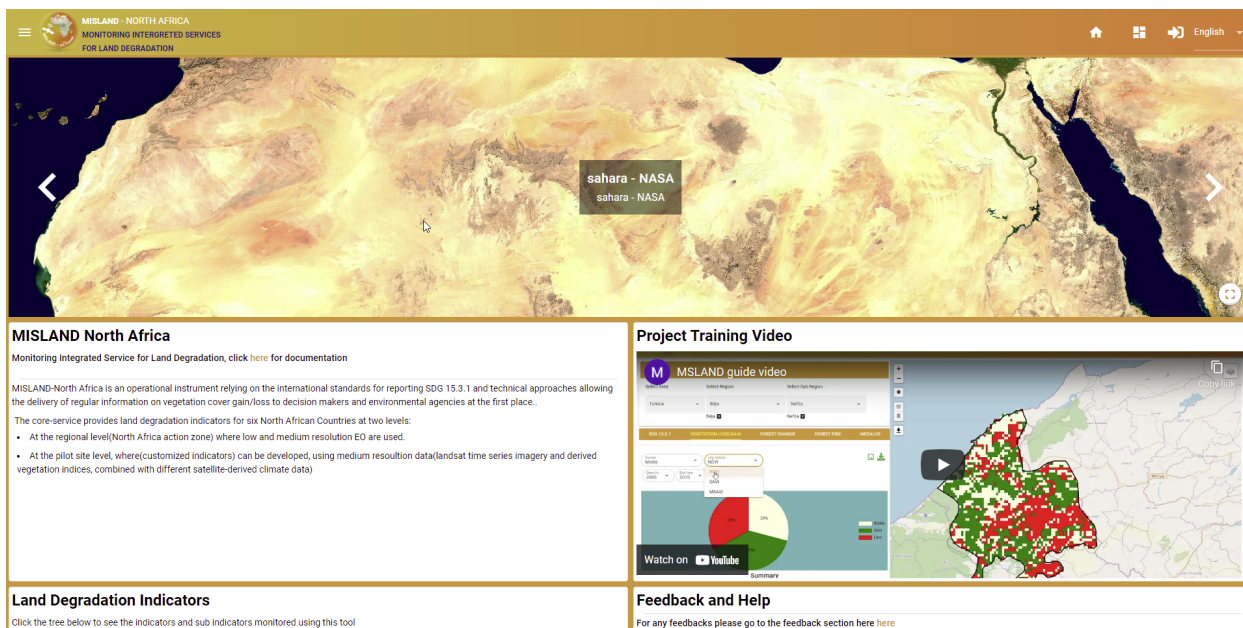
Fig. 1: Misland Homepage
