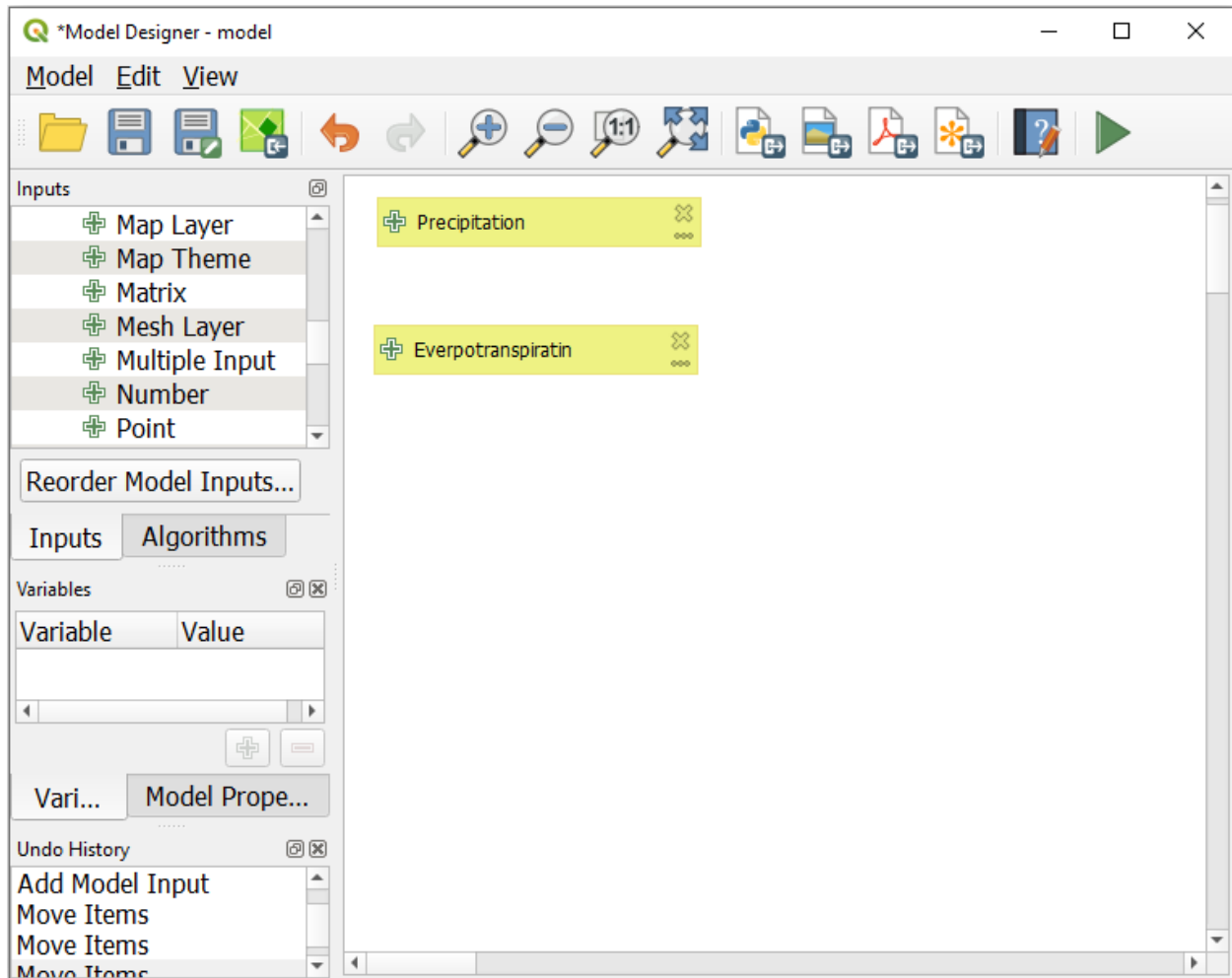
Fig. 4: Model Inputs
